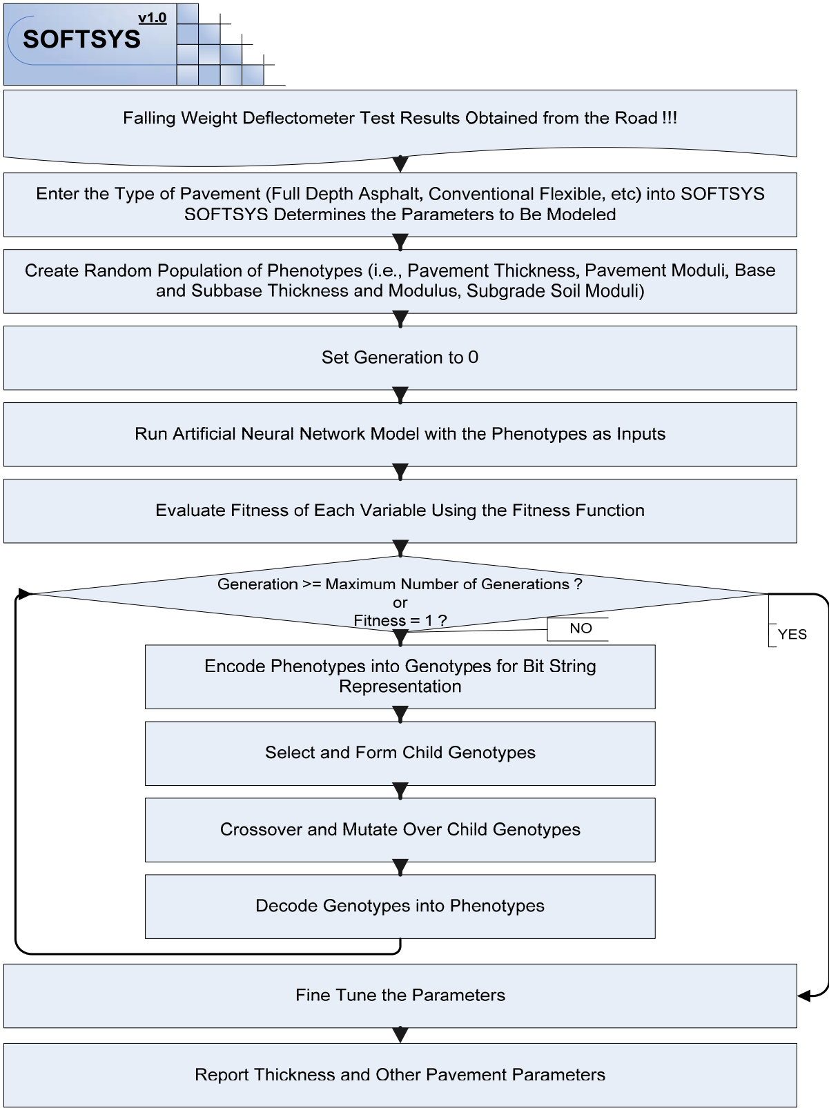
Figure 4-2. SOFTSYS algorithm.
